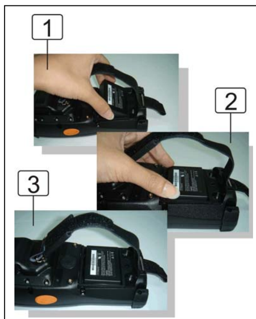
Figure 2-9 Insert the battery pack
