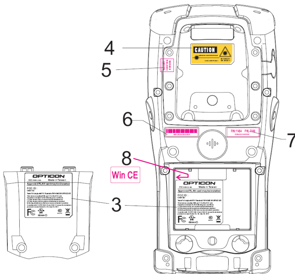
Figure 1-2 PHL-7100 Labeling (Rear view)
