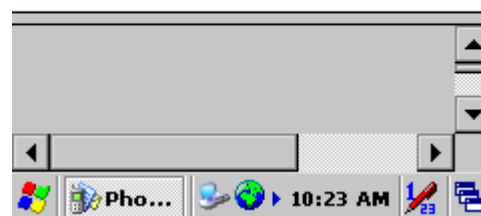
Figure 6-3 Inbox
