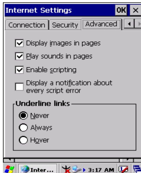
Figure 3-53 Internet Settings
