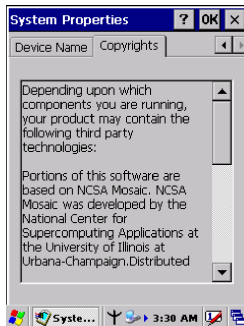
Figure 3-86 System Properties
