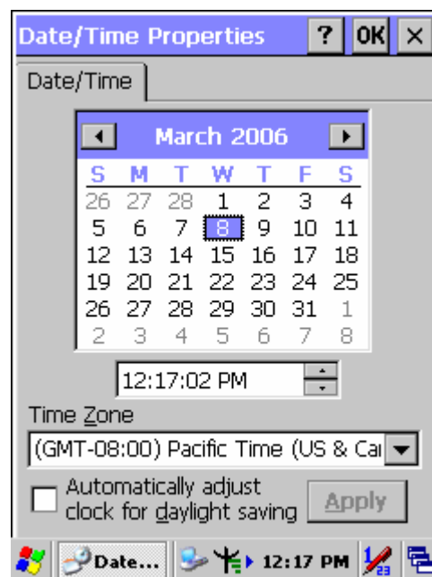
Figure 2-18 Date/Time properties
