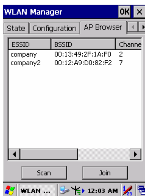
Figure 2-21 WLAN Manager
