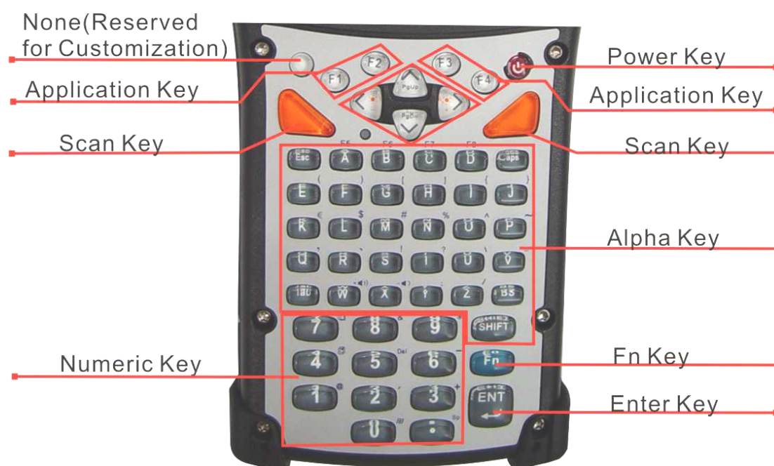
Figure 2-16 PDT Keypad
