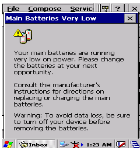
Figure 3-76 Power
