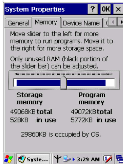
Figure 3-84 System Properties
