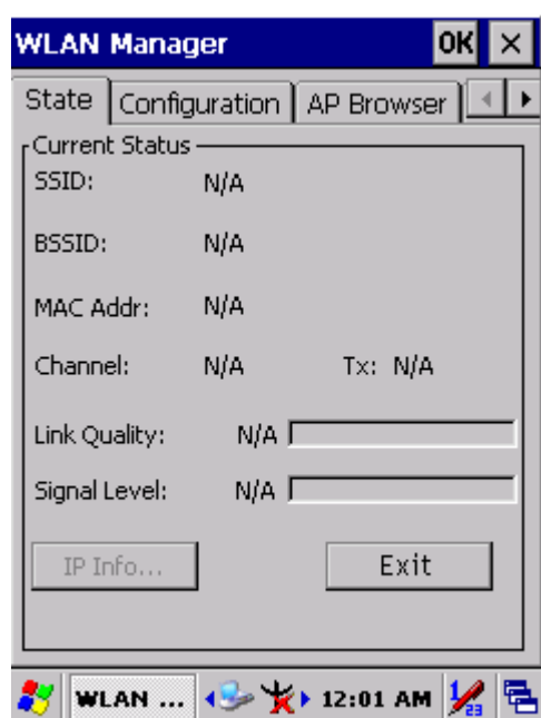
Figure 2-20 WLAN Manager
