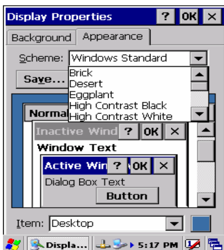
Figure 3-47 Display properties
