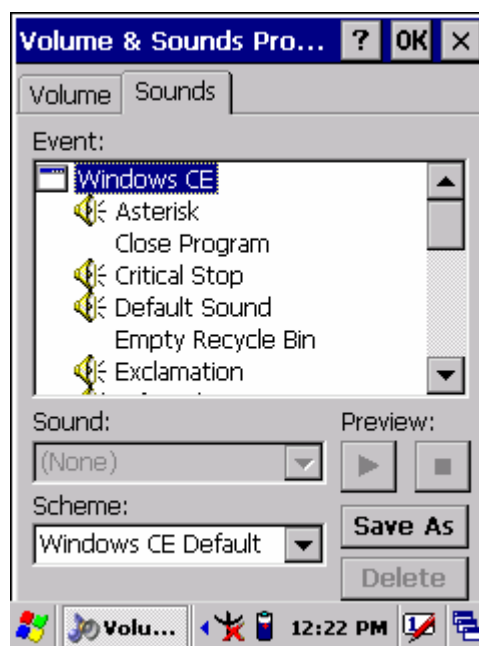
Figure 3-88 Volume & Sound
