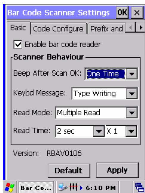
Figure 3-2 Basic Tab
