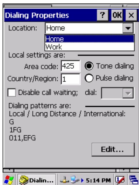
Figure 3-39 Dialing Properties
