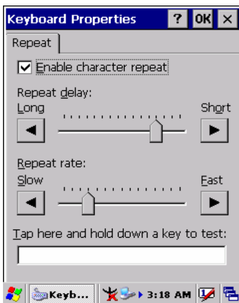
Figure 3-54 Keyboard Properties
