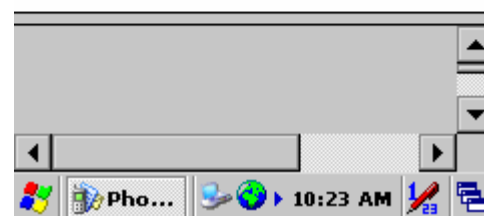
Figure 6-4 Outbox
