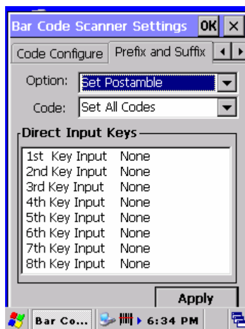
Figure 3-10 Postamble option
