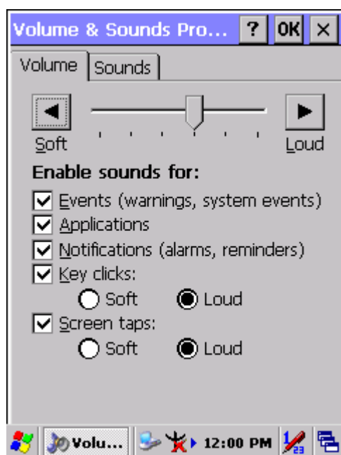
Figure 3-87 Volume & Sound
