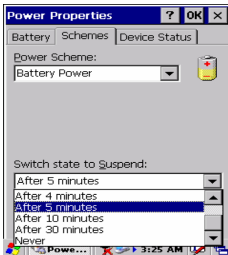
Figure 3-74 Power
