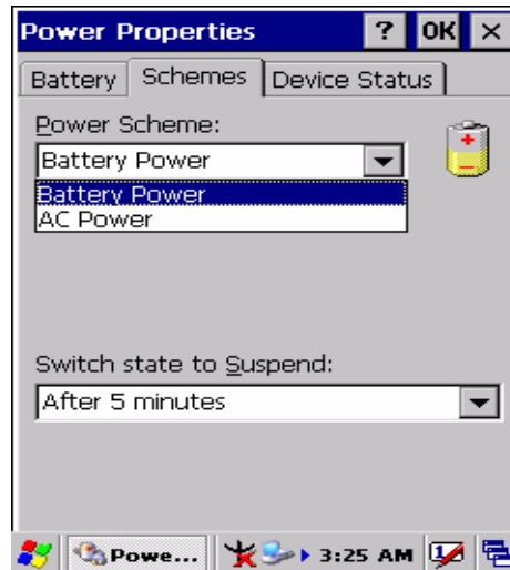
Figure 3-73 Power
