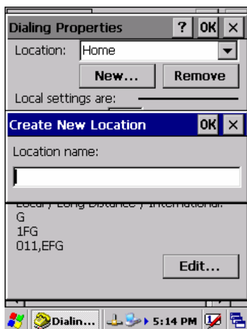
Figure 3-41 Dialing Properties
