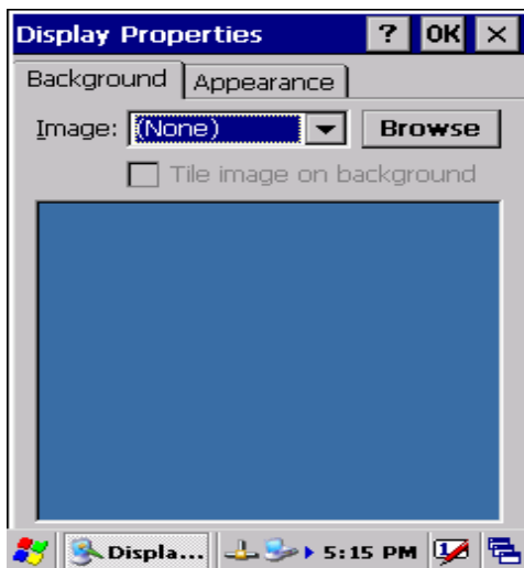
Figure 3-43 Display properties
