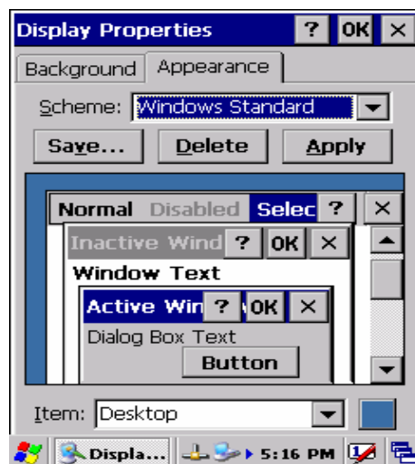
Figure 3-46 Display properties
