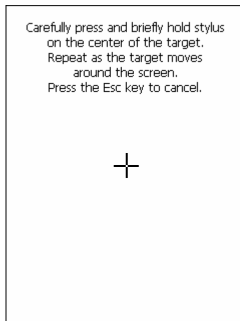
Figure 3-82 Stylus Properties
