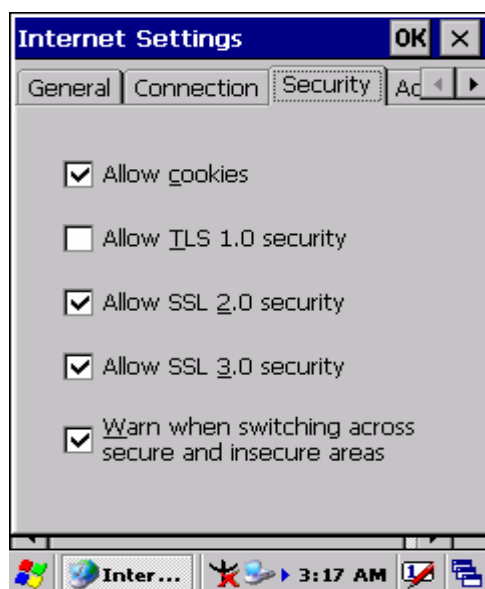
Figure 3-52 Internet Settings
