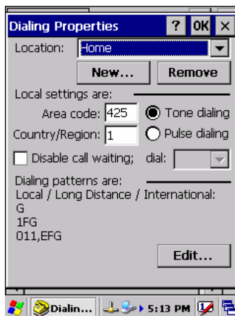
Figure 3-40 Dialing Properties
