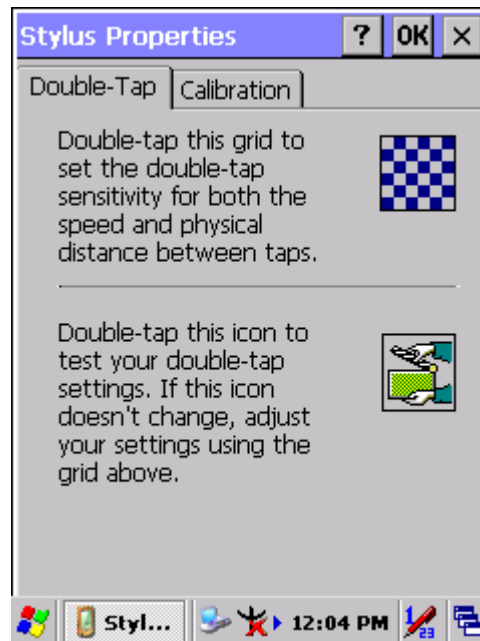
Figure 3-80 Stylus Properties
