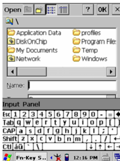
Figure 3-38 Fn-Key Settings
