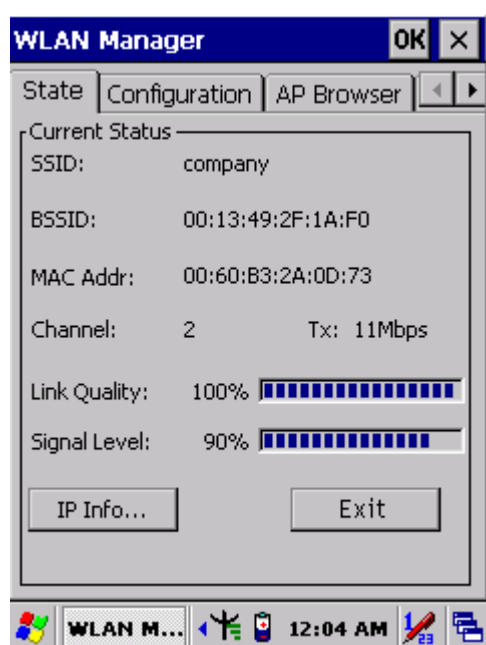
Figure 2-22 WLAN Manager
