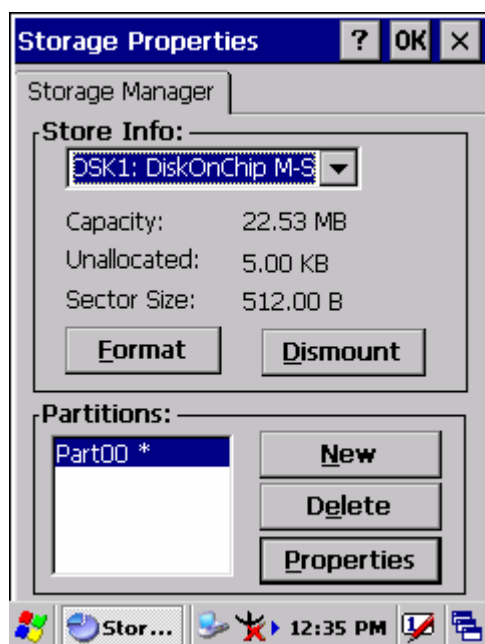
Figure 3-78 Storage Manager
