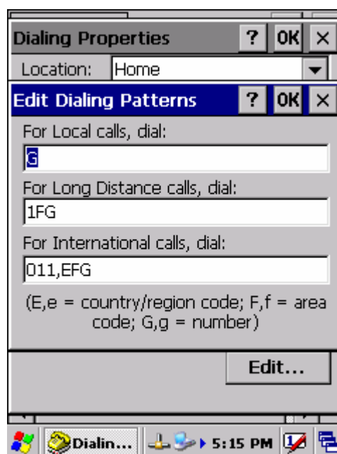
Figure 3-42 Dialing Properties
