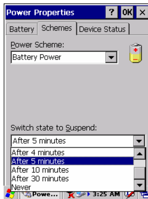
Figure 2-24 Schemes Tab
