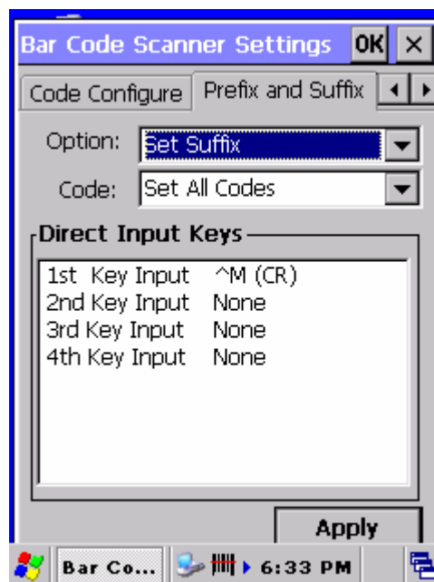
Figure 3-8 Suffix option
