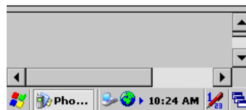
Figure 6-5 Sent box
