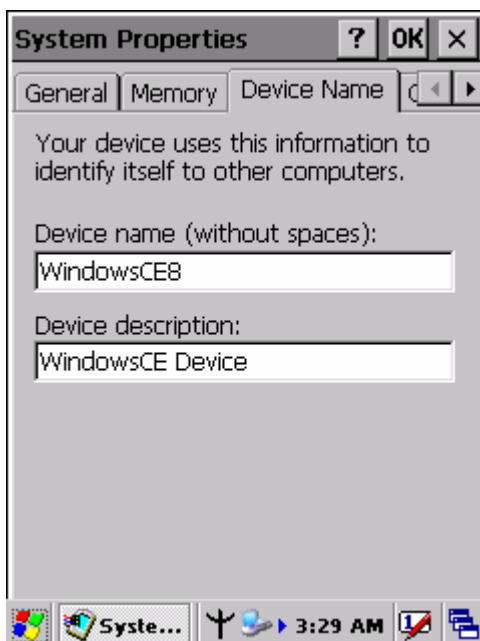
Figure 3-85 System Properties
