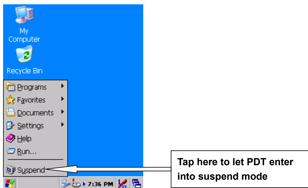
Figure 2-25 Suspend
