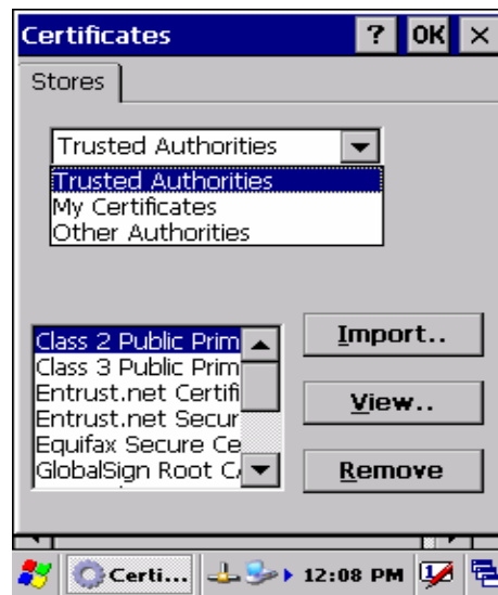
Figure 3-27 Certificates
