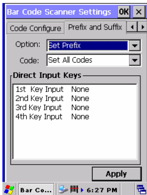
Figure 3-7 Prefix option
