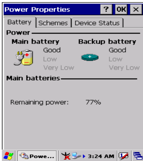
Figure 3-72 Power
