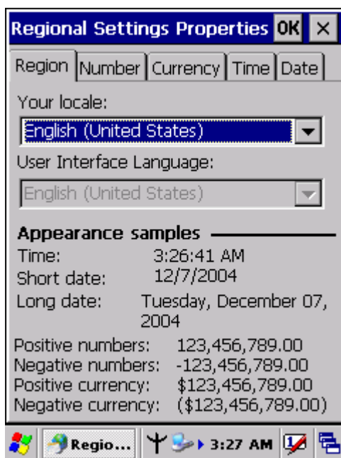
Figure 3-77 Regional Settings
