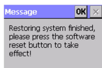
Figure 3-36 Restore OK
