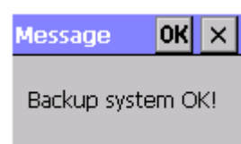
Figure 3-33 Backup Restore
