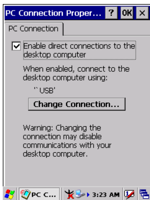
Figure 3-70 PC Connection
