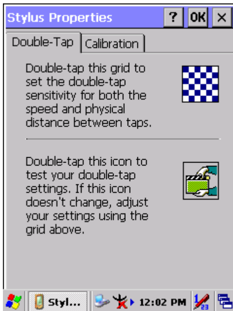
Figure 3-79 Stylus Properties
