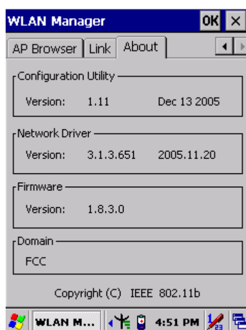
Figure 2-23 WLAN Manager
