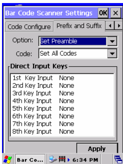
Figure 3-9 Preamble option
