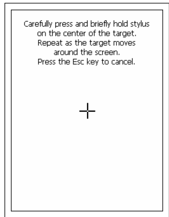
Figure 2-14 Calibration
