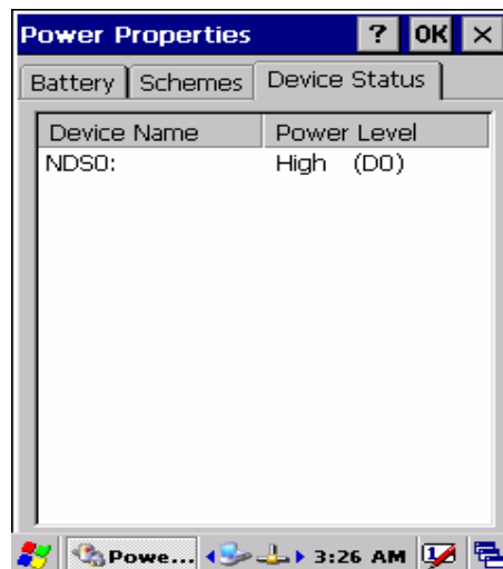
Figure 3-75 Power
