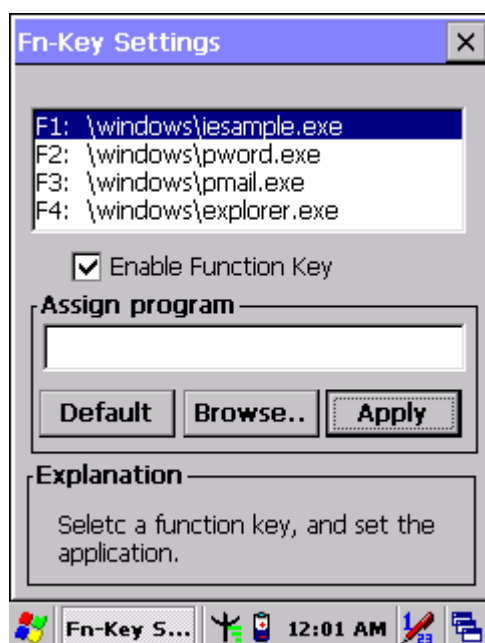
Figure 3-37 Fn-Key Settings
