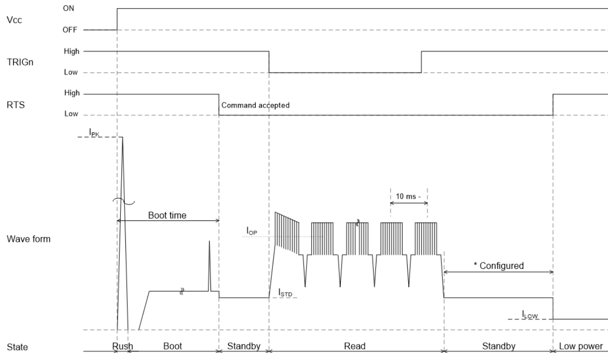
Figure 4: Current Waveform
